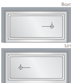
SHOWER BASE 60" x 30" x 3 5 / 8 "
